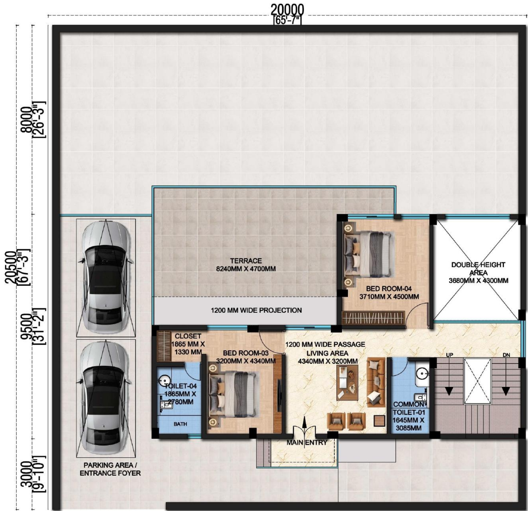
First Floor-95.875 sqm
